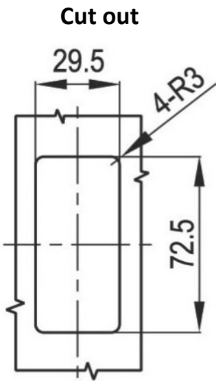
Panel cutout
