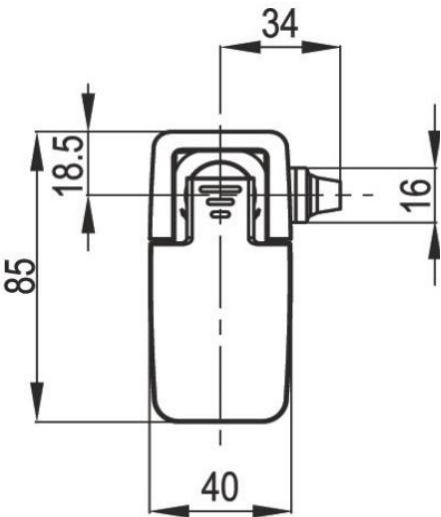
Non-locking
