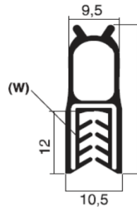
PA7400071-000 **mm. 1 a 2,5 SILICONE COMPACT + METAL
