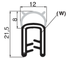
PA7400022-000 **mm. 2 a 4 SILICONE COMPACT + METAL
