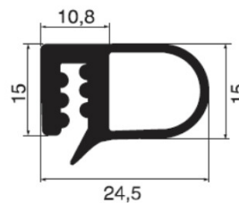
PA7400073-000 **mm. 2 SILICONE COMPACT
