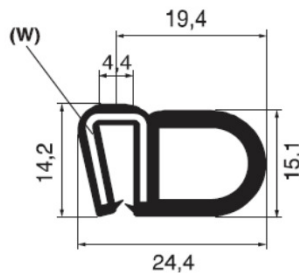
PA7400062-000 **mm. 1,5 a 3 SILICONE COMPACT + METAL
