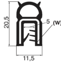
PA7400069-000 **mm. 1,5 a 3 SILICONE COMPACT + METAL
