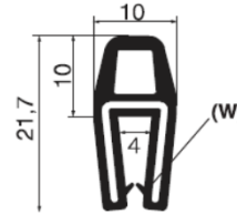
PA7400061-000 **mm. 1 a 3 SILICONE COMPACT + METAL
