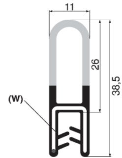
PA7400046-000 **mm. 1,5 a 3 SILICONE COMPACT + SPONGE + METAL
