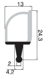
PA7400019-000 SILICONE COMPACT SPONGE
