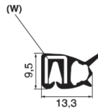
PA7400067-000 **mm. 1 a 2 SILICONE COMPACT + METAL
