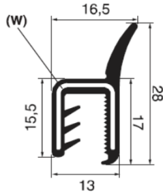
PA7400065-000 **mm. 5 a 6 SILICONE COMPACT + METAL DIN5510
