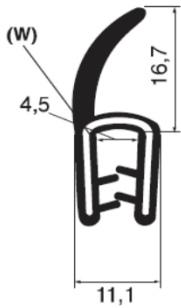
PA7400076-000 **mm. 1,5 a 3 SILICONE COMPACT + METAL
