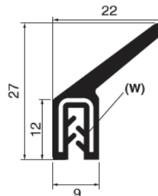
PA7400064-000 **mm. 1 a 2 SILICONE COMPACT + METAL
