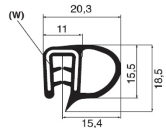
PA7400070-000 **mm. 1,5 a 3 SILICONE COMPACT + METAL
