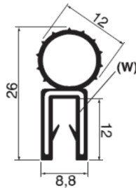
PA7400078-000 **mm. 2 a 3,5 SILICONE COMPACT + METAL
