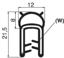
PA7400045-000 **mm. 2 a 4 SILICONE COMPACT + METAL
