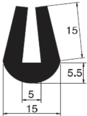
PA7100559-000 EPDM
