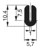
PA7200228-000 PVC
