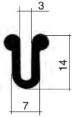
PA7100895-000 EPDM
