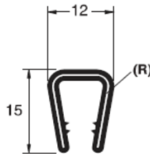
PA7200295-000 **mm. 6 a 8 PVC
