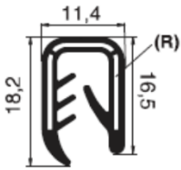
PA7200406-000 **mm. 4 a 6 PVC
