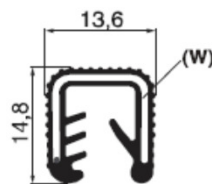
PA7102035-000 **mm. 5 a 6 EPDM
