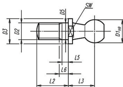
Form C with threaded pin and SW
