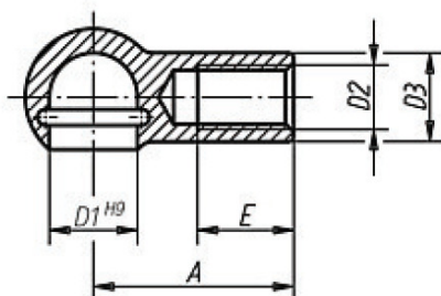
Form A with snap ring
