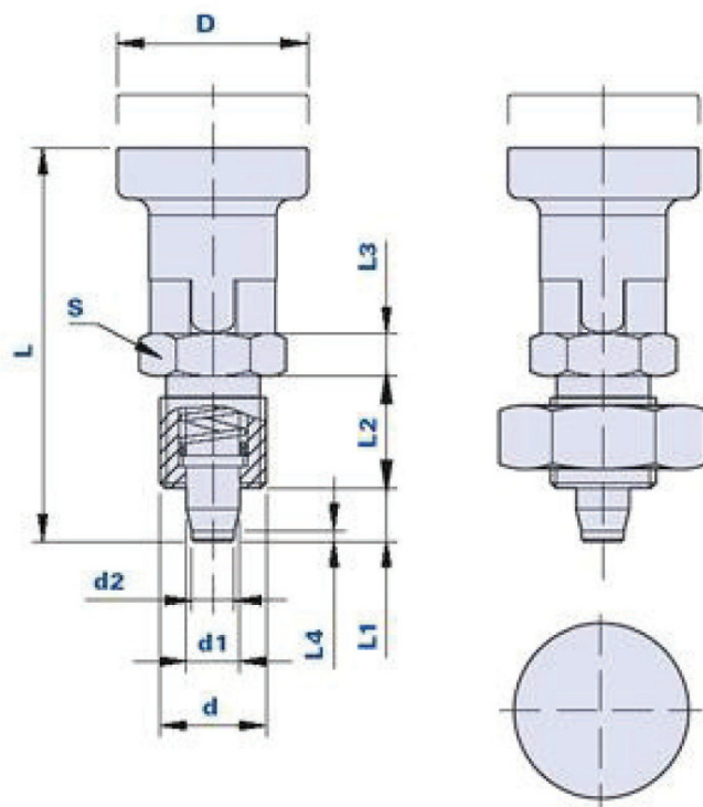
PA6805-5-M10x1.25 (Without nut)
