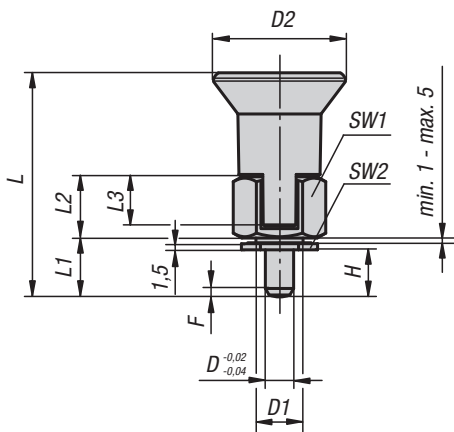
Form C lockout type
