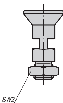
Form D lockout type with locknut
