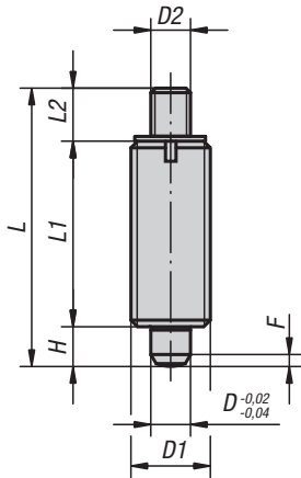
Form J with threaded pin without locknut
