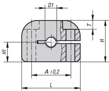
Form B Fastening hole vertical to thread
