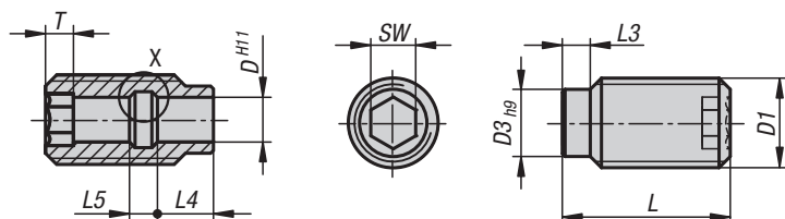
view "X"
