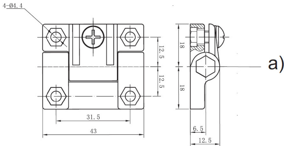
Screw adjustment
